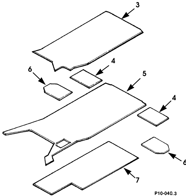
FOUR-DOOR CAB
