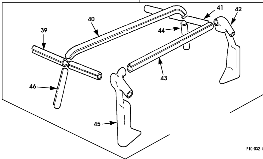
Figure 10-37. Soft Top Support Structure, Model 90 (Sheet 1 of 2).
