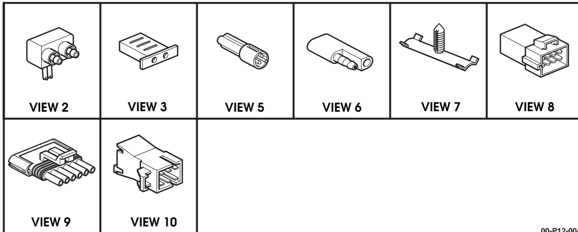
Figure 12-53. Harness Assembly, Slant-Back Cargo Door, Model 91.
