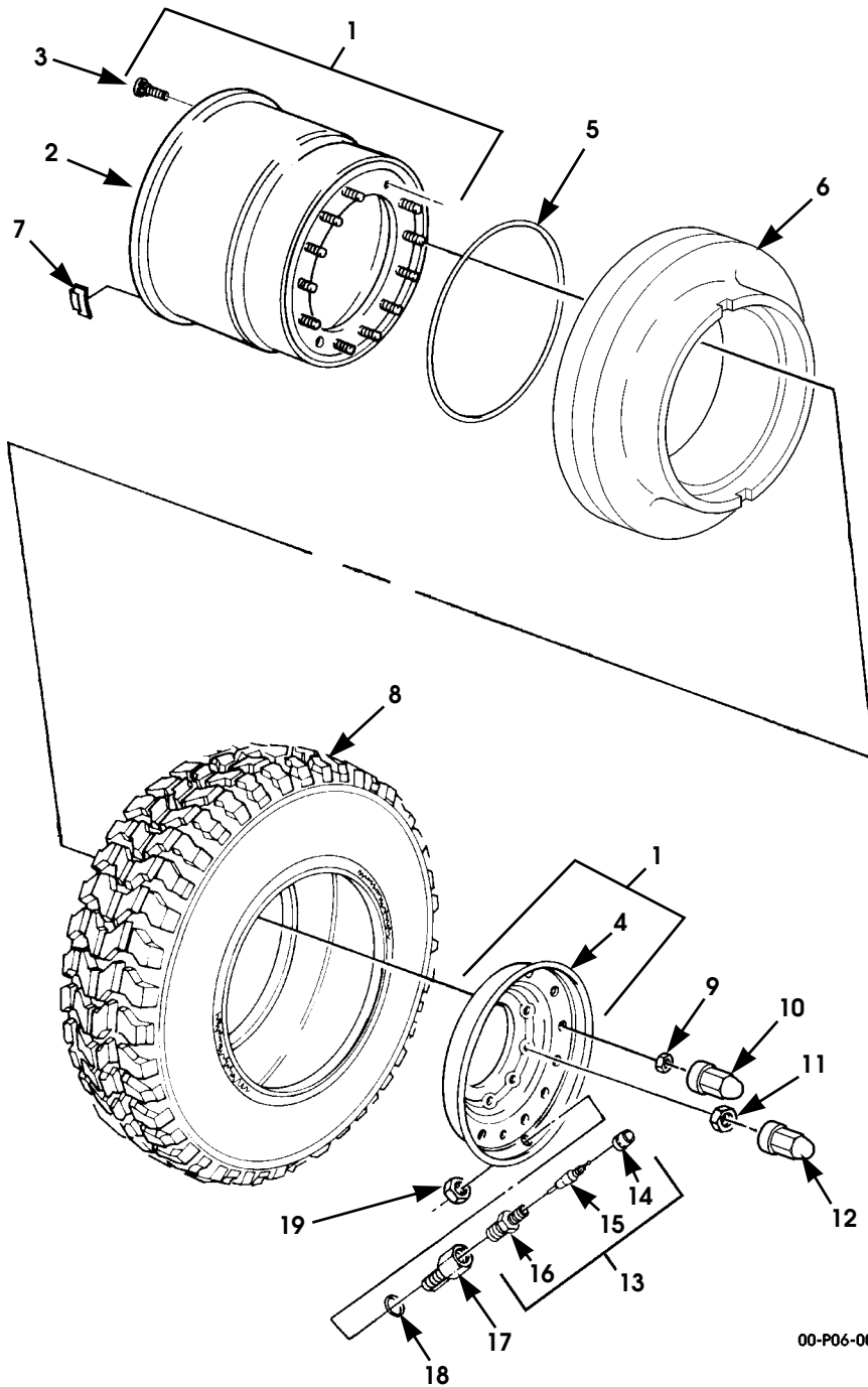
Figure 6-1. Wheel, Tire, and Runflat Assembly, Two-Piece Rim.
