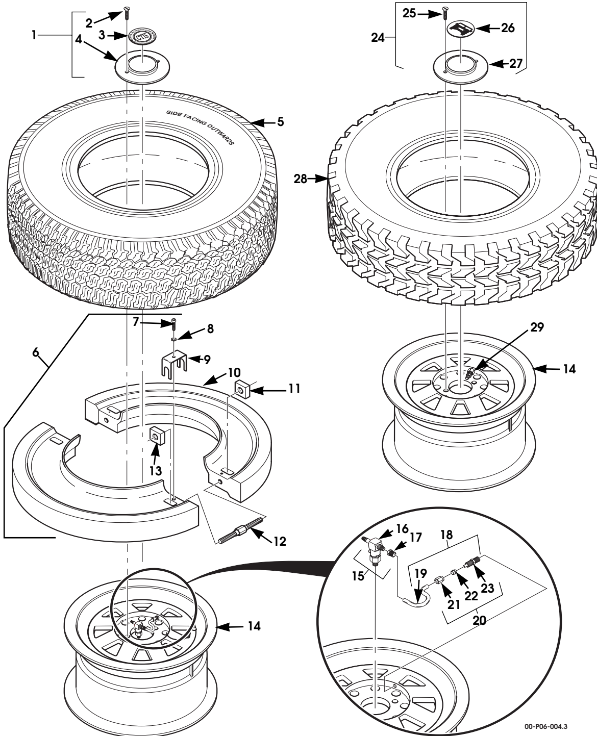
Figure 13-18. Wheel, Tire, and Runflat Assembly, One-Piece Aluminum Rim, 16.5" (Optional).
