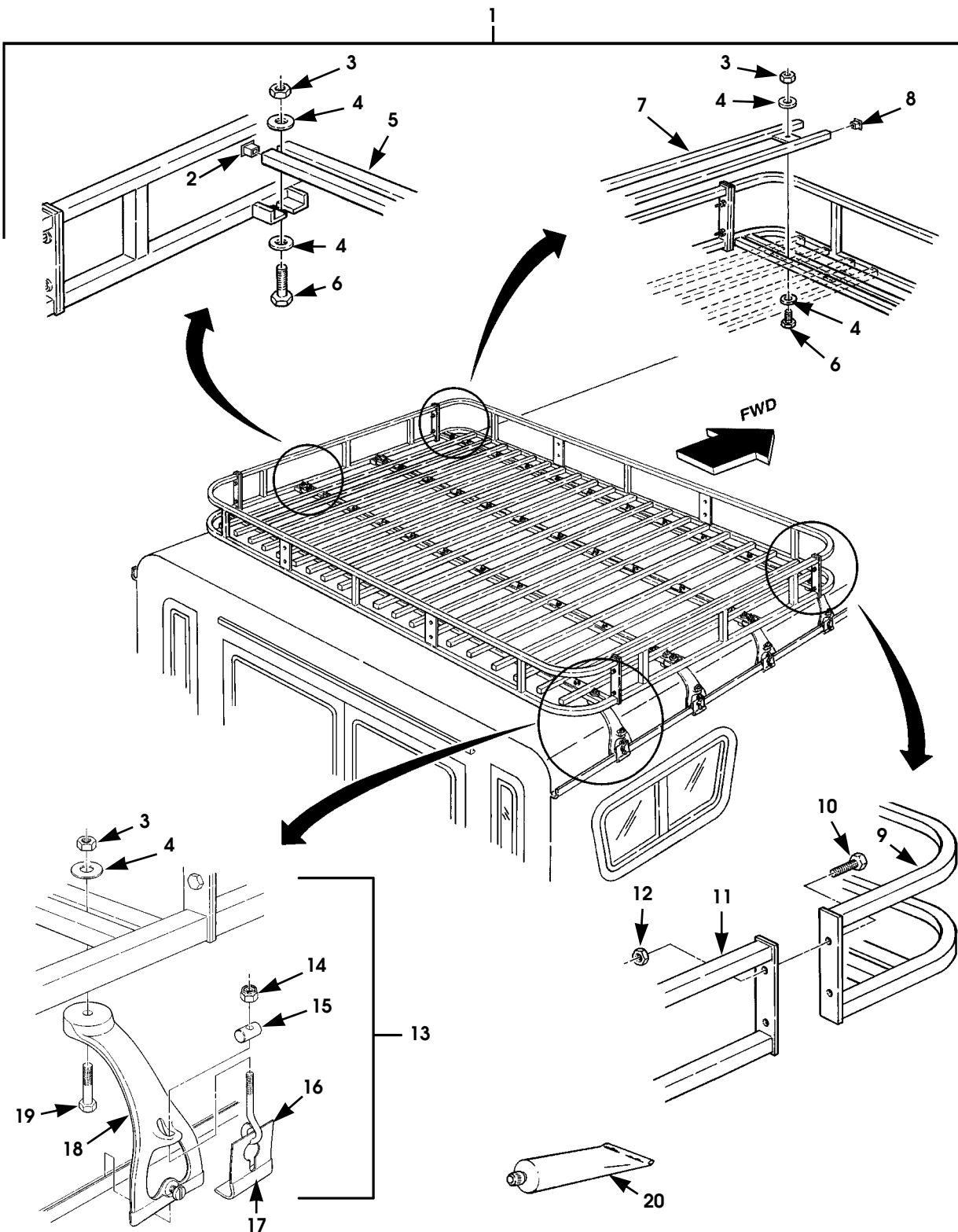
Figure 13-60. Roof Rack Kit, Steel, Square Tube.
