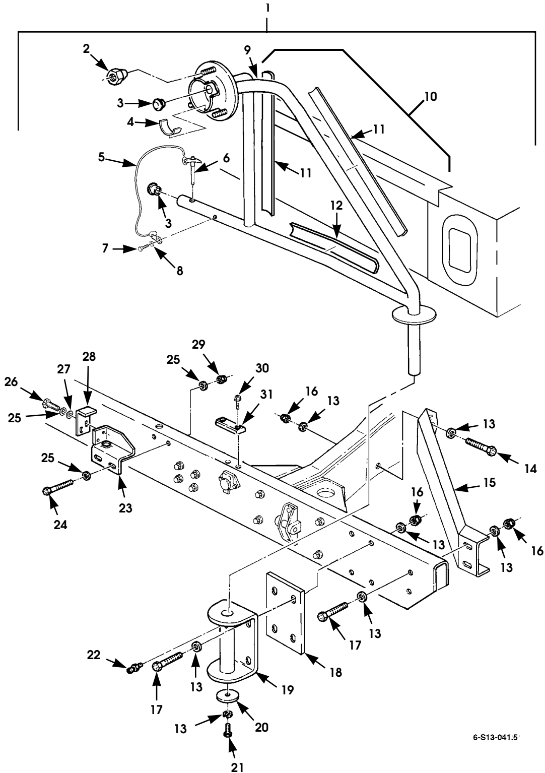
Figure 13-11. Spare Tire Carrier Kit, Swing-Away (Steel Wheels Only).
