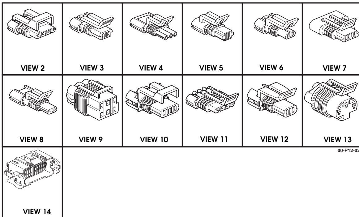
Figure 12-57. Engine Harness Assembly, GM.
