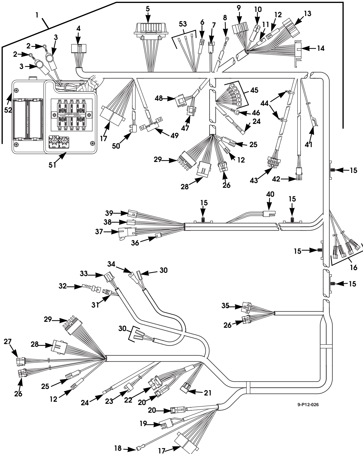
Figure 12-51. Cross Body Harness (Sheet 1 of 3).
