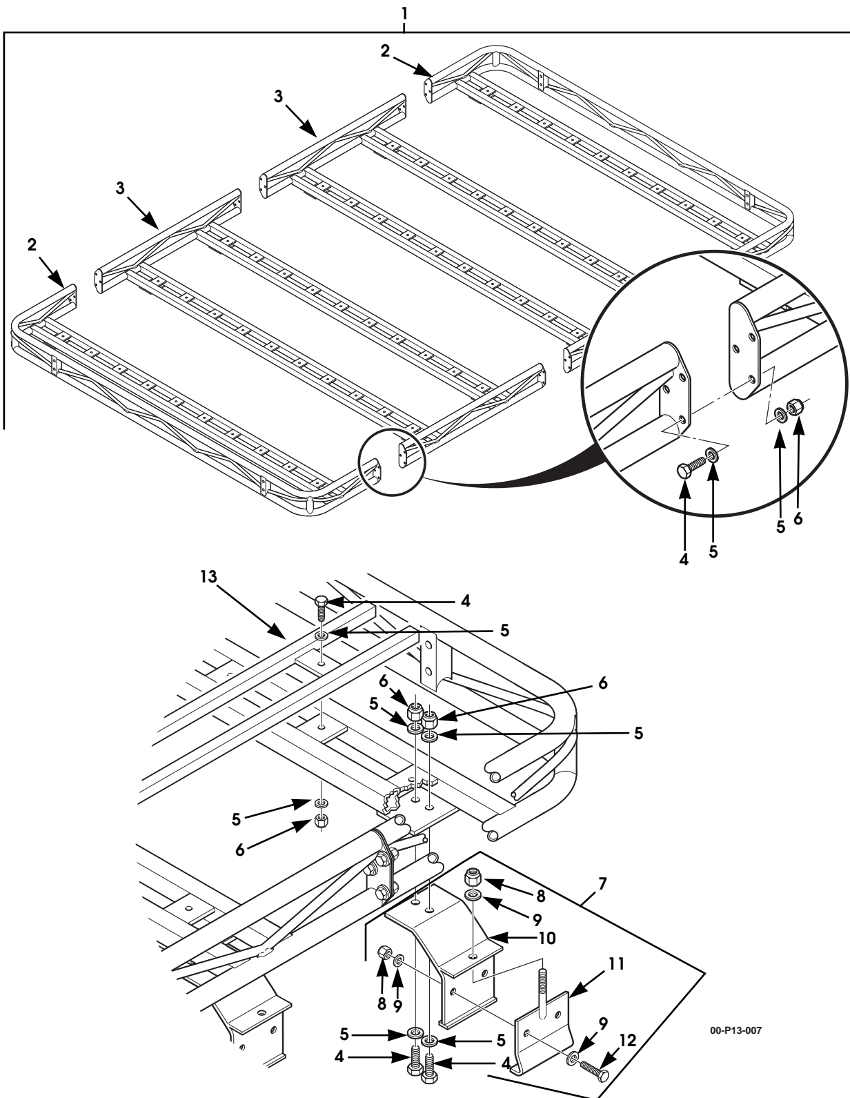
Figure 13-61. Roof Rack Kit, Aluminum, Round Tube.
