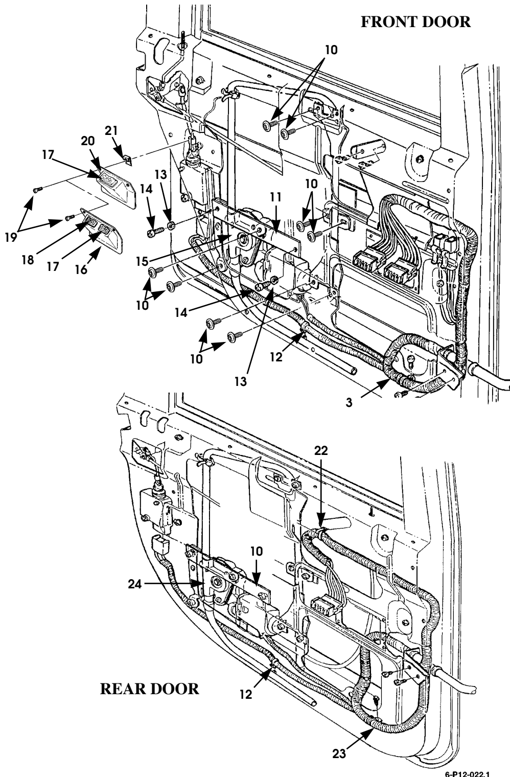
Figure 12-36. Power Window (Sheet 2 of 2).
