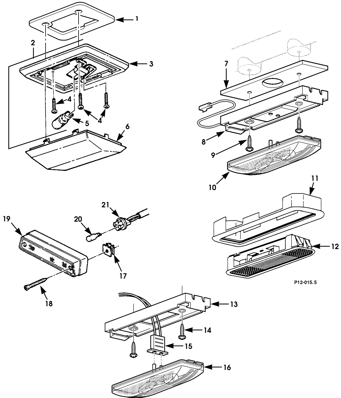
Figure 12-13. Interior Dome Lights.
