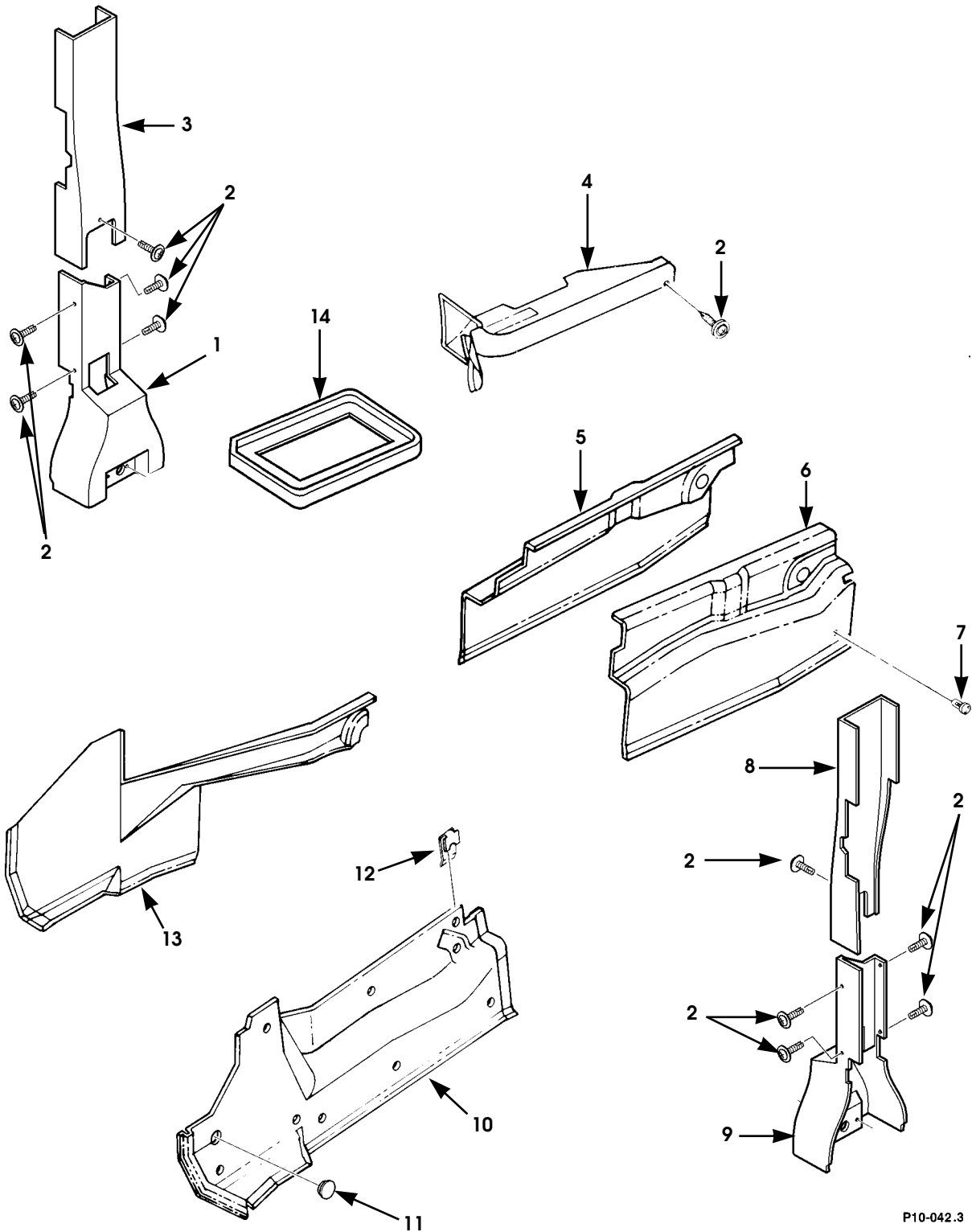
Figure 10-49. Inner Kick Panels and Miscellaneous Trim Panels.
