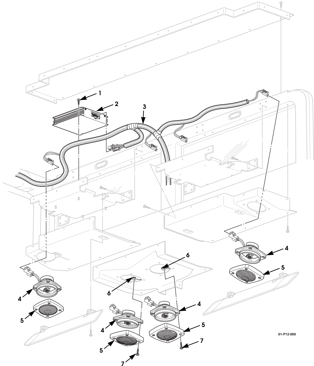
Figure 12-27. Monsoon System, Soft-Top.
