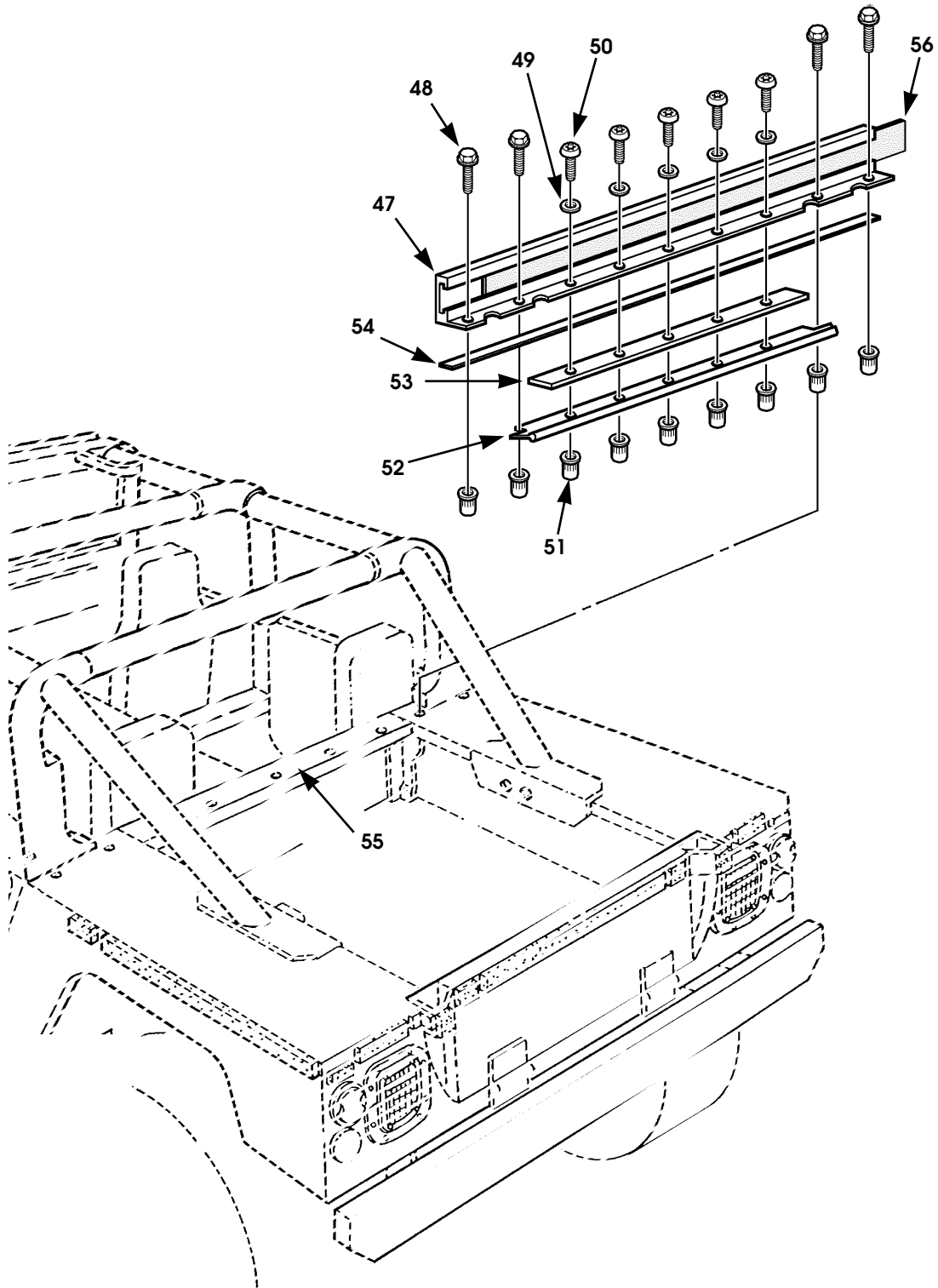
Figure 10-37. Soft Top Support Structure, Model 90 (Sheet 2 of 2)
