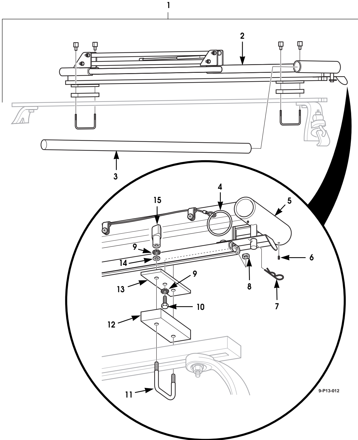
Figure 13-56. Roof Rack Kit, Side Load.
