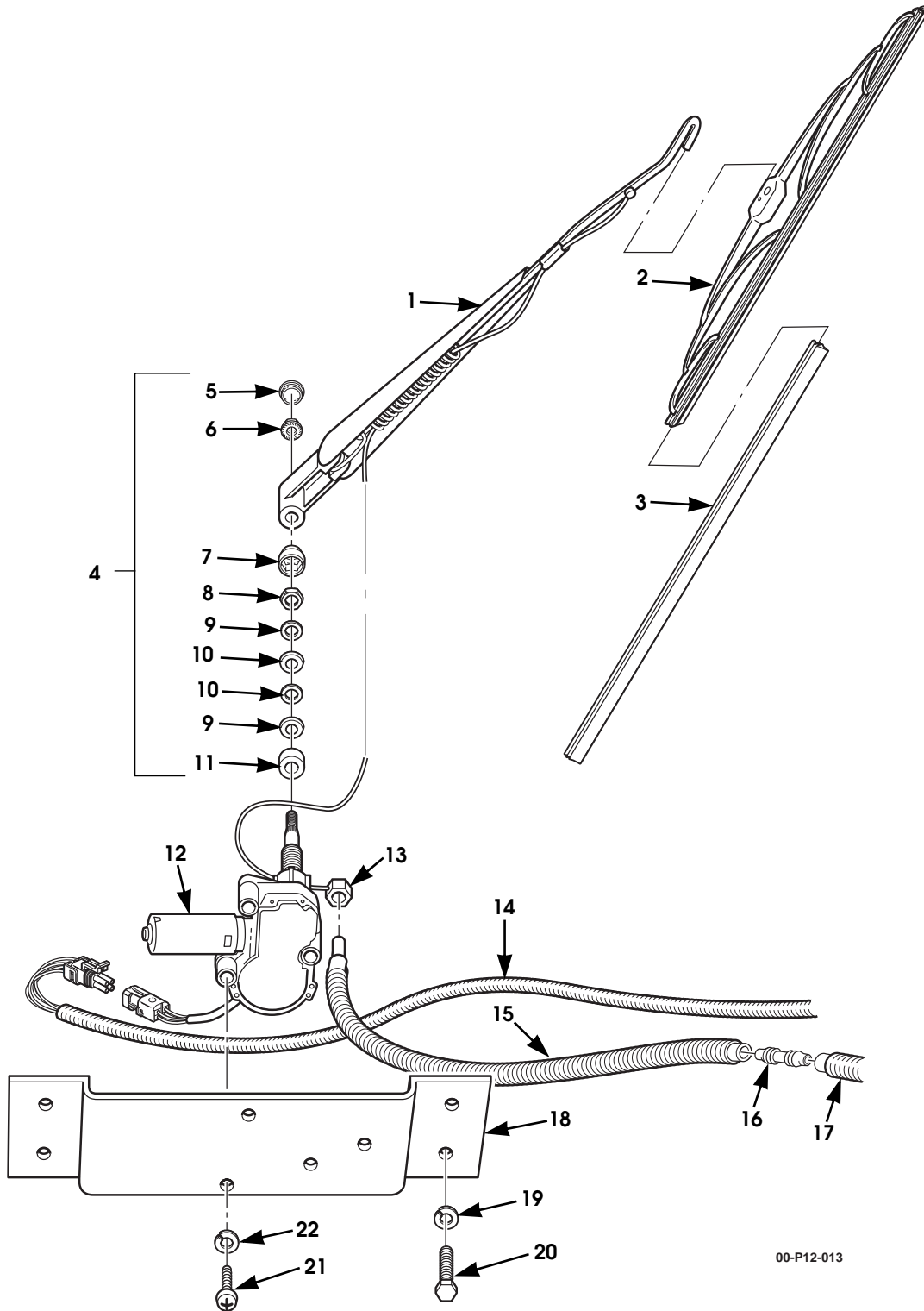
Figure 12-7. Wiper Motor And Blade, Slant-Back Rear Window.
