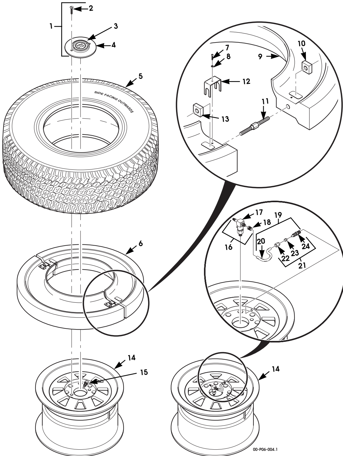
Figure 6-3. Wheel, Tire and Runflat Assembly, 17", One-Piece Aluminum (Optional).
