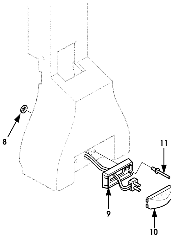
Figure 12-14. Interior Courtesy Lights, Underhood Light, and Door Jamb Switch
