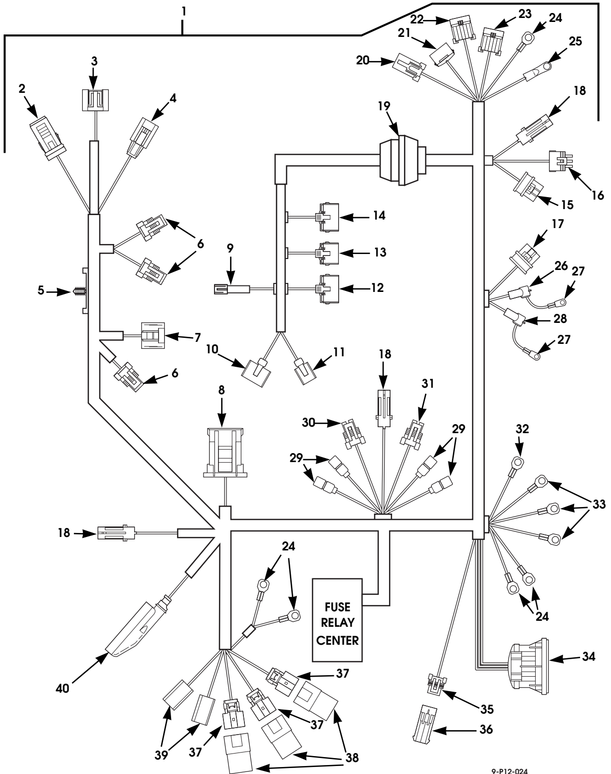
Figure 12-52. Cowl Top Harness (Sheet 1 of 2).
