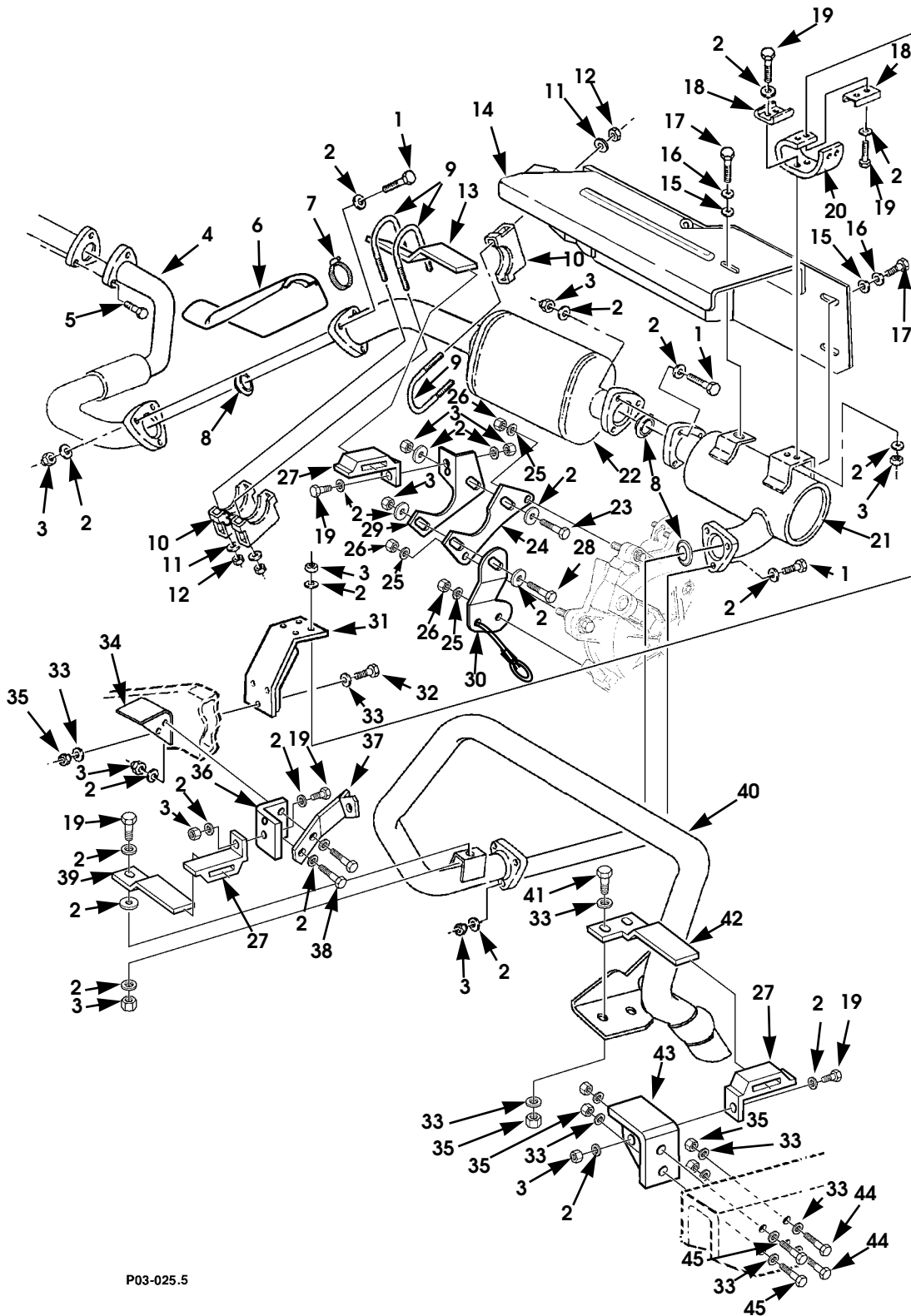
Figure 3-13. Exhaust Pipes and Related Parts.
