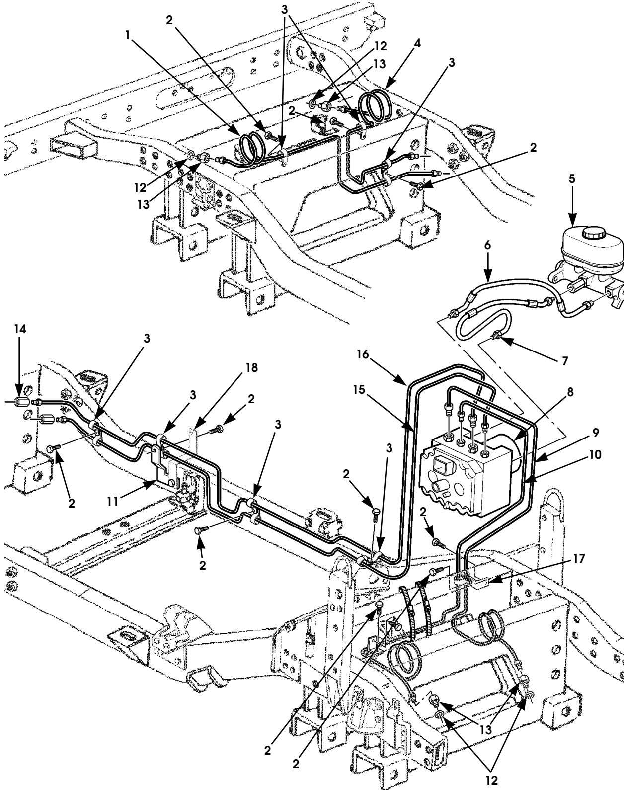
Figure 7-7. Brake Lines.
